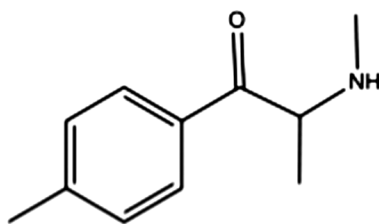
(a) Mefedrona
